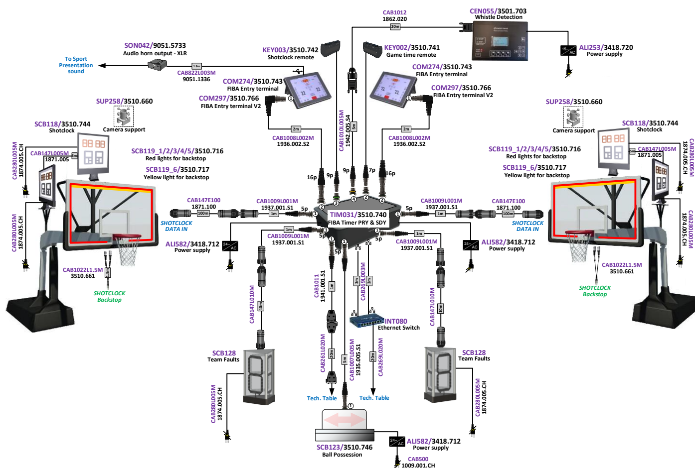
Figure 2 – FIBA T&amp;S System Scheme (Event)
