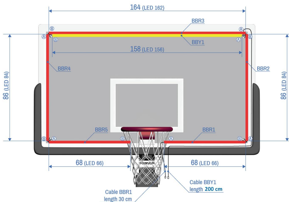
Figure 16 - BBLight dimensions
