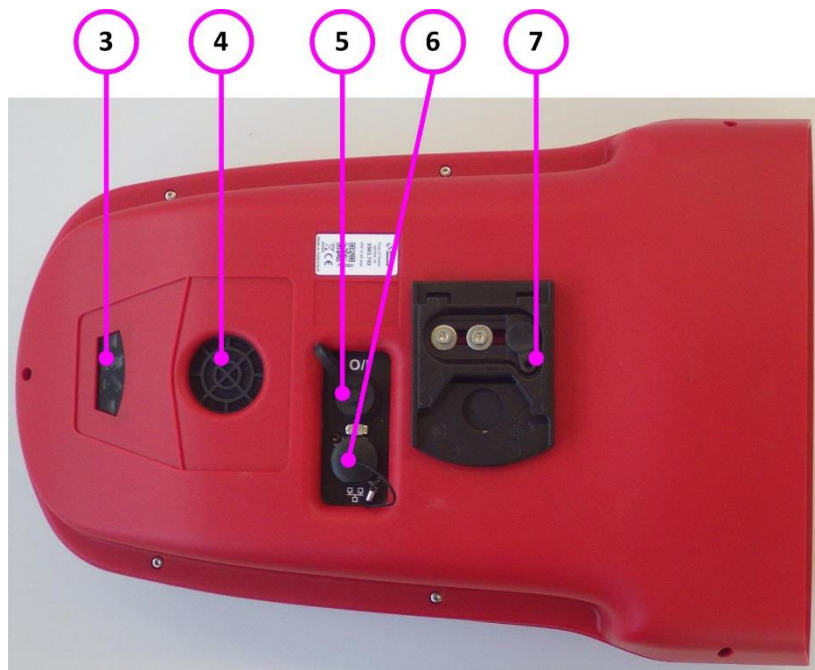
Figure 2 – MYRIA bottom view
