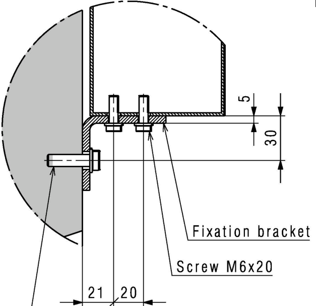
Fixation Bracket
