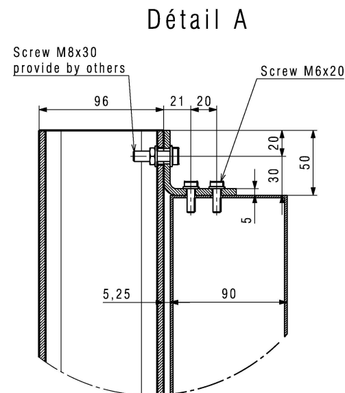
Fixation Bracket
