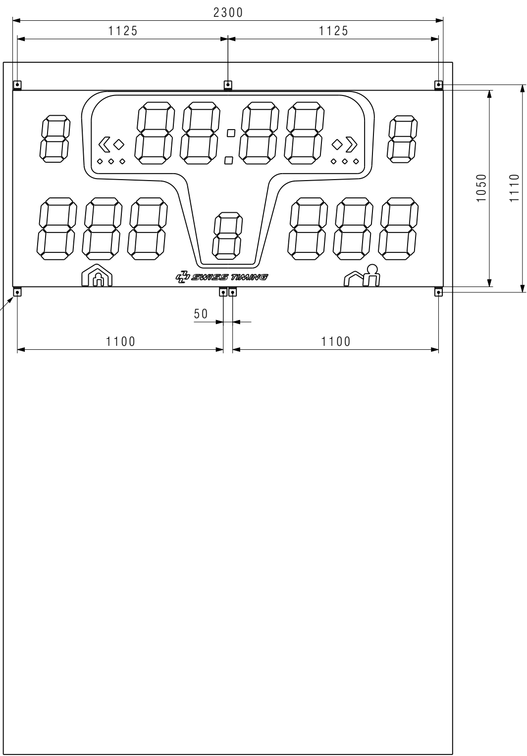
Fixation Bracket
