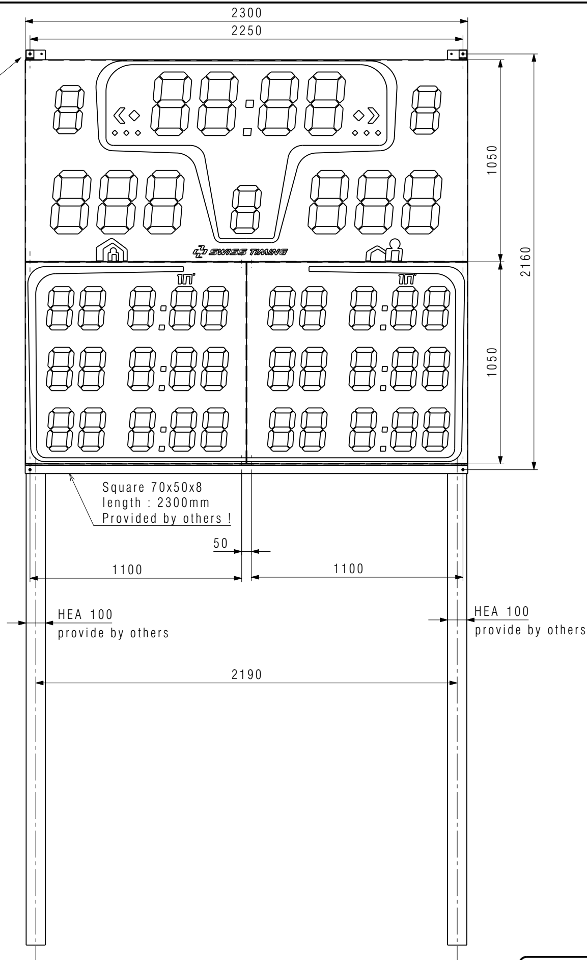
Fixation Bracket
