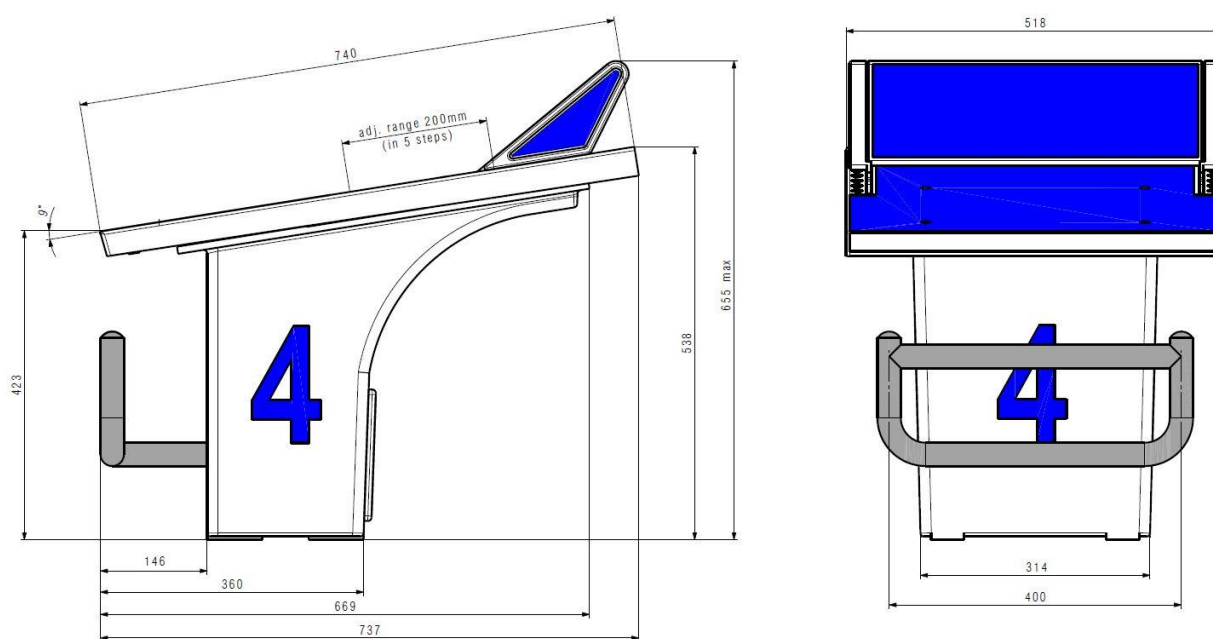
Figure 4 – Technical specifications
