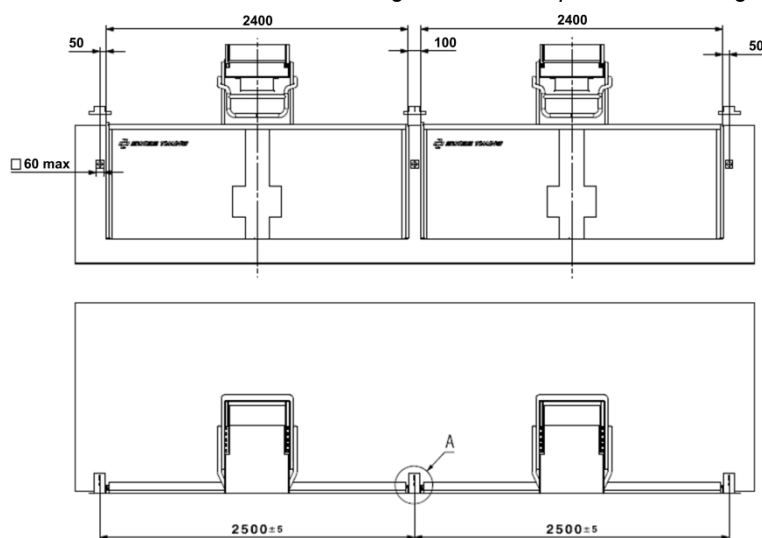
Figures 4 - Touchpad 240x90 / Angle bracket mounting
