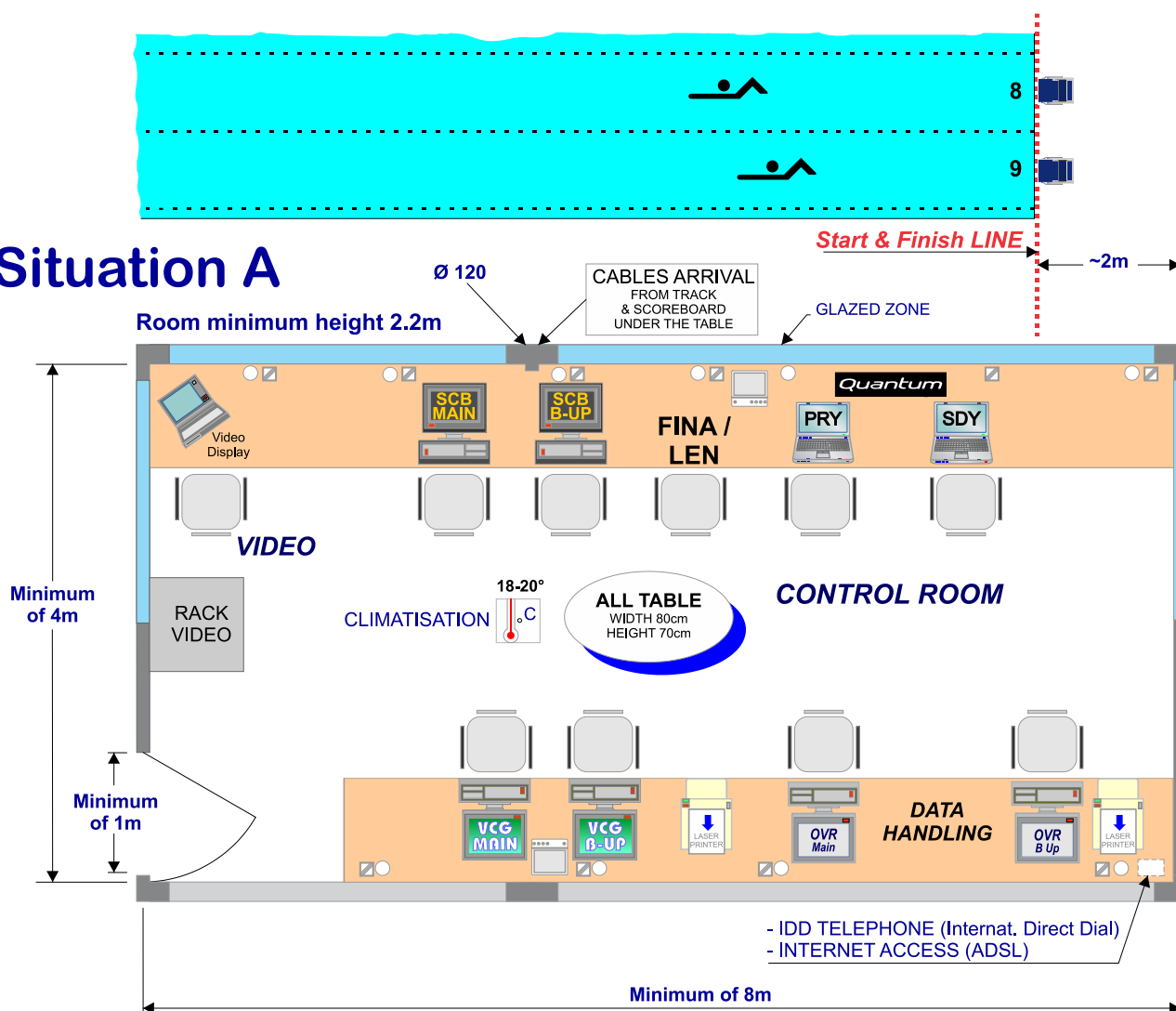
Figures 2 – Timing room layout 1
