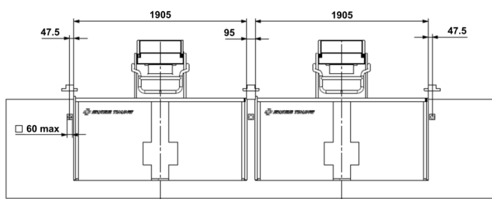
Figures 6 - Touchpad 190x90 / Angle bracket mounting
