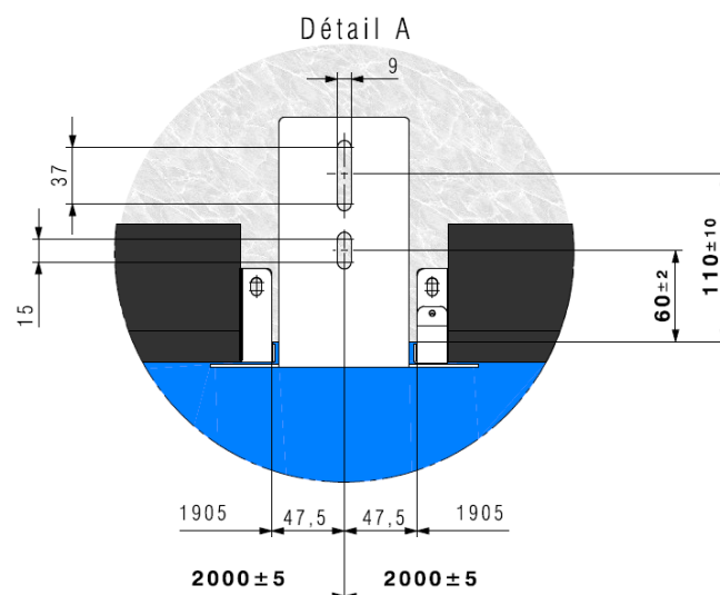
Figures 6 - Touchpad 190x90 / Angle bracket mounting
