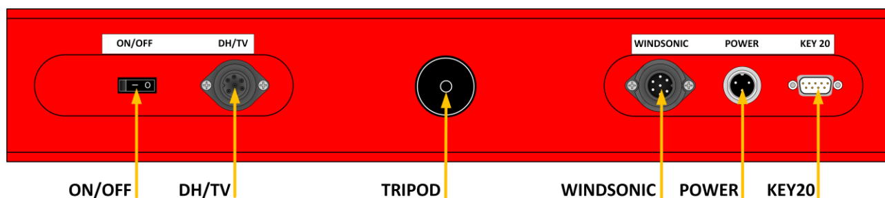
Figure 2 – Bottom view
